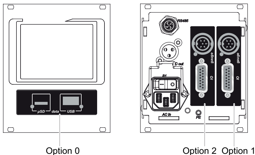
Fig. 3: OmniControl addresses, example
